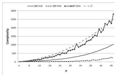
Figure 1: Computational Results
